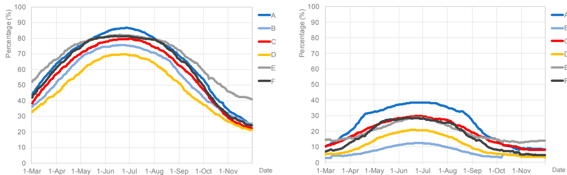
Figure 8. Percentages of ground-level surface with direct sunlight for three or more hours ( left ) and six or more hours ( right ) from March to November for study sites A to F when FAR is 2.5.
