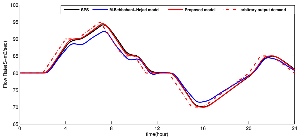
Figure 6. Inlet flow rate changes with time.
