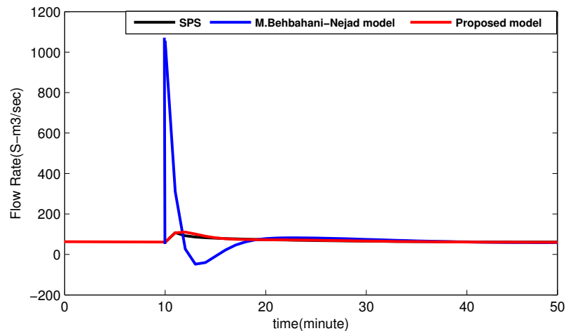
Figure 5. Inlet flow rate changes with time.
