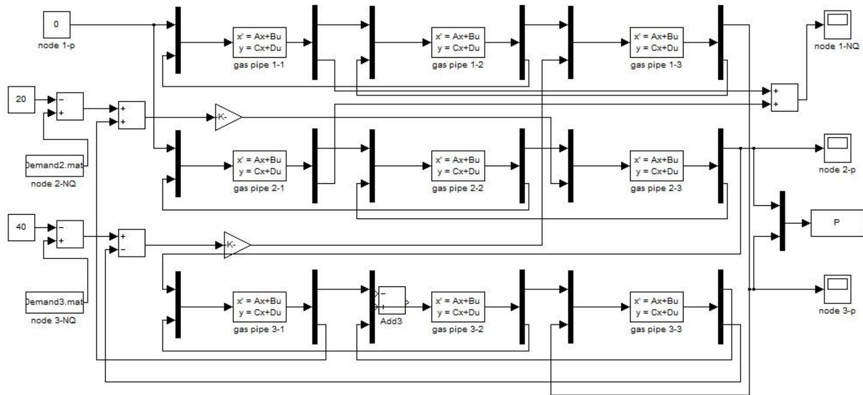
Figure 9. MATLAB-Simulink model of the typical network.
