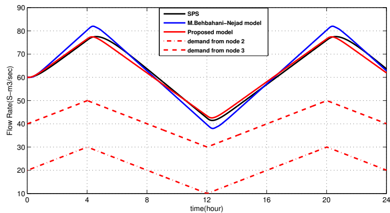
Figure 10. Demands for node 2 and node 3 and inlet flow rate for node 1.
