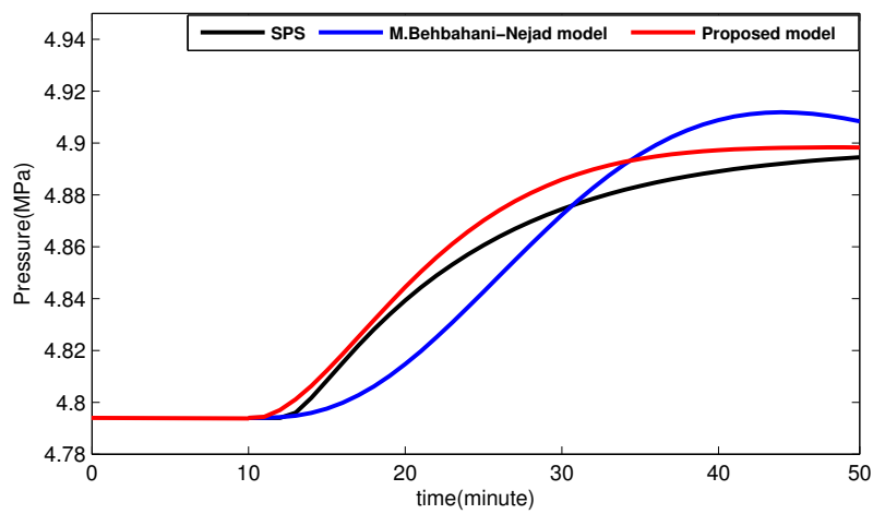
Figure 4. Outlet pressure changes with time.
