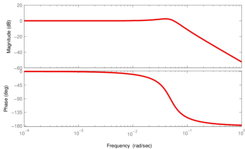
Figure 2. Bode plot of \Delta m_{out} and \Delta m_{in} in Equation (24).
