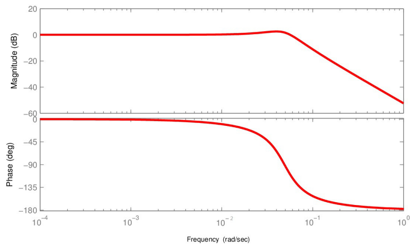
Figure 1. Bode plot of \Delta p_{in} and \Delta p_{out} in Equation (23).
