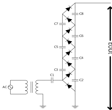
Figure 8. Cockcroft Walton circuit and transformer.
