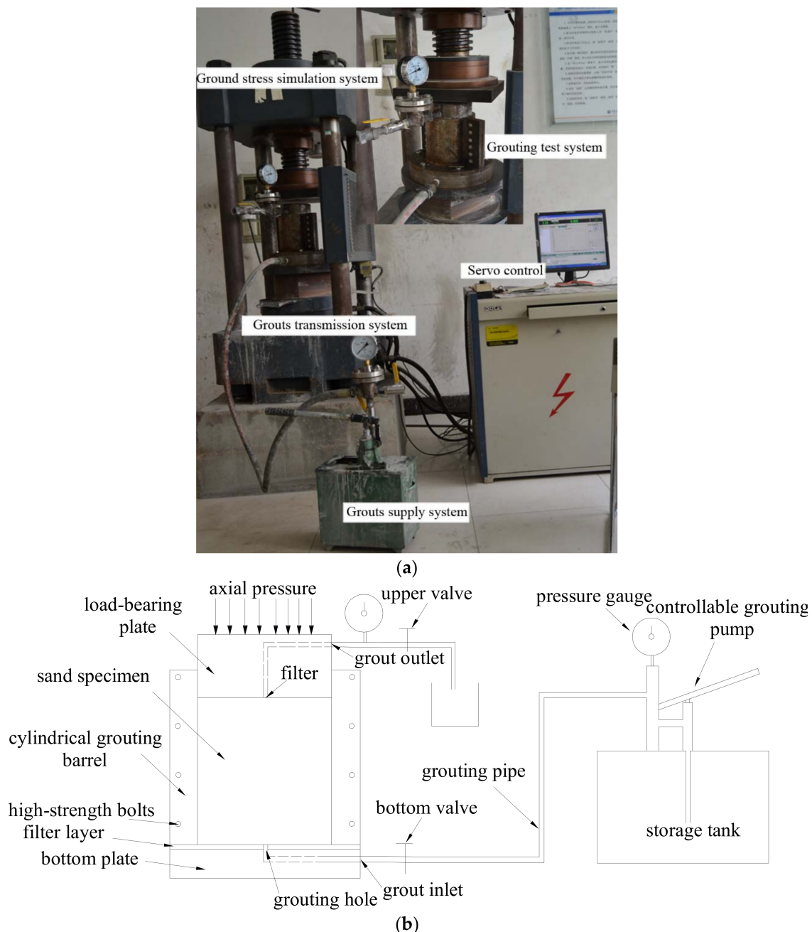
Figure 2. (a) Grouting experimental setup and (b) detailed schematic layout of the grouting test system.
