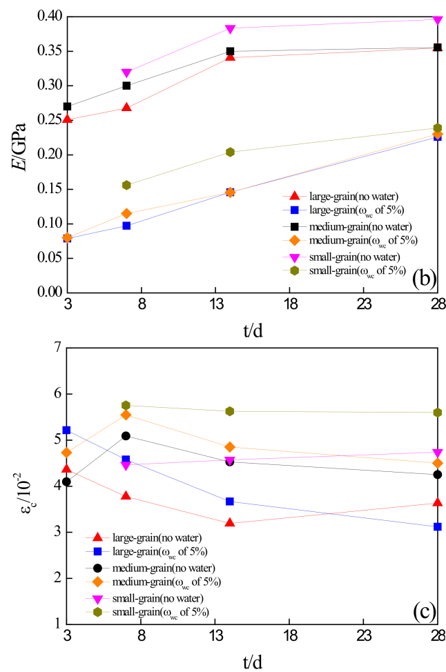
Figure 4. Different average values of mechanical parameters versus curing time. (a) \sigma_c , (b) E , (c) \varepsilon_c .
