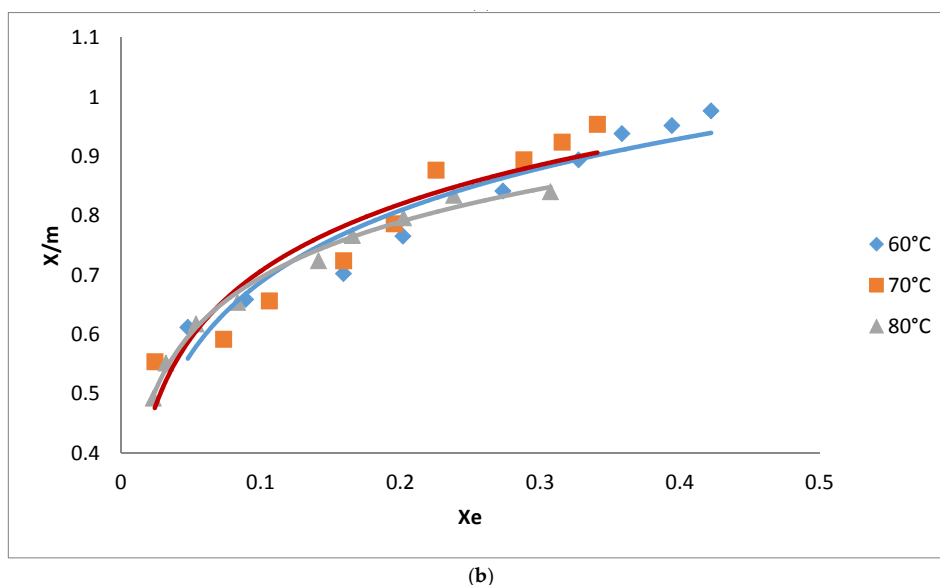
Figure 4. (a) Adsorption isotherm for the removal of pigments from oil using AC from cotton; (b) Adsorption isotherm for the removal of pigments from oil using AC from neem.
