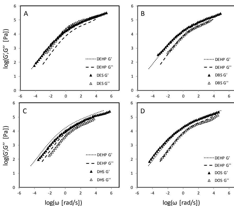
Figure 3. Dynamic elastic moduli of succinate plasticizers showing the effect of plasticizer chain length on the storage ( G' ) and loss ( G'' ) moduli of PVC blends with DEHP as compared to blends with: (A) diethyl succinate (DES); (B) dibutyl succinate (DBS); (C) dihexyl succinate (DHS) and (D) dioctyl succinate (DOS). All PVC–plasticizer blends were 40 phr.
