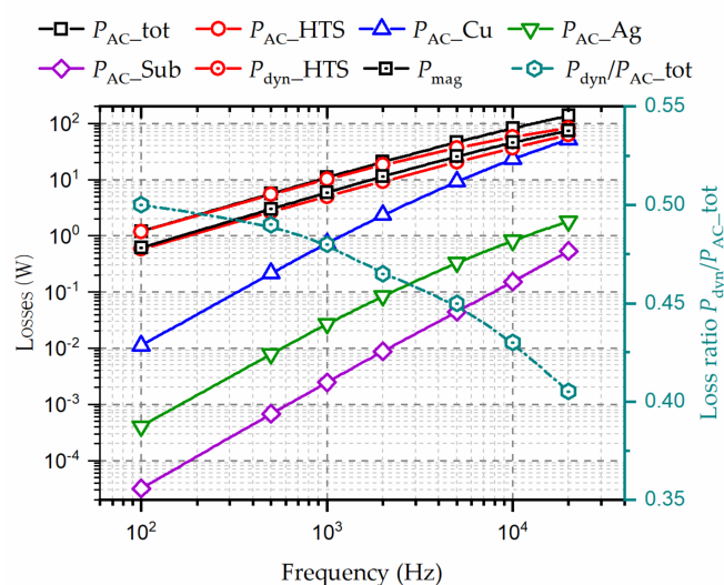
Figure 6. Dynamic loss, magnetization loss, AC losses in different layers, and loss ratio P_{\text{dyn}}/P_{\text{AC-tot}} of the 2 \times 12 HTS double pancake racetrack coil at different frequencies. The AC field frequency, f , ranges from 100 Hz to 20 kHz. The DC transport current I_t = 50 A. B_{\text{ext}} = 50 mT [23].
