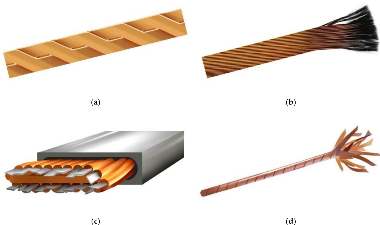
Figure 16. Pictures of Roebel and Rutherford-type cables: (a) Roebel cable fabricated from HTS CCs, adapted from [225]; (b) Rutherford cable made from round superconducting wires, adapted from [226]; (c) Twisted flat HTS cable made from HTS CCs, adapted from [229]; (d) CORC ® wire, adapted from [224].
