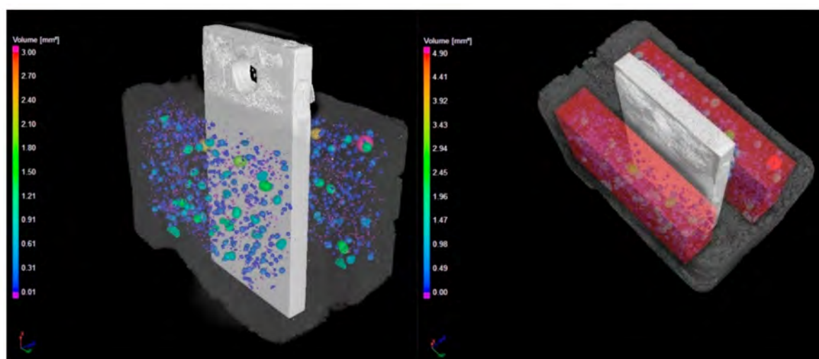
Figure 8. Computed tomography scan of steel/Variodur specimen in pristine form (control specimen). The pores are imaged (left) and quantified in the red area (right).
