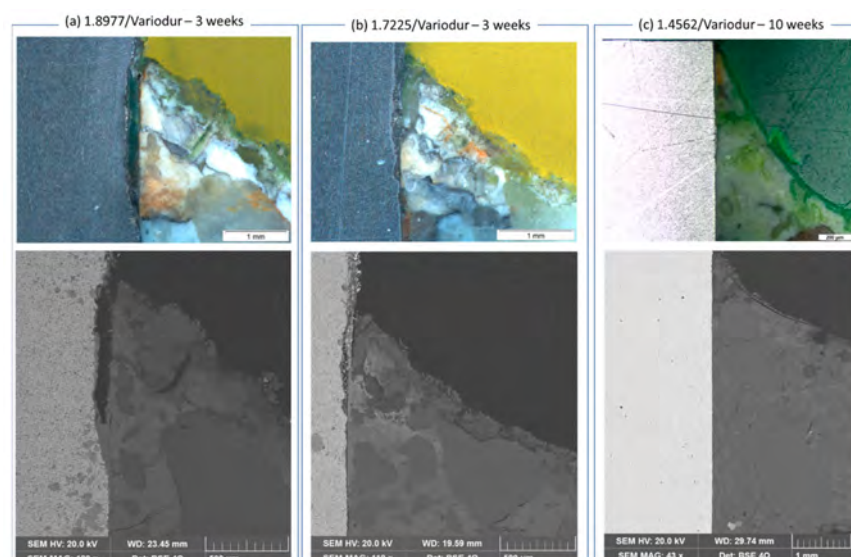
Figure 10. Crevice corrosion at the steel/Variodur interface after exposure to 333 K, 10 MPa, and synthetic aquifer fluid. Crevice formation from the top. The upper row images were taken by a stereomicroscope, while the image (right) below was taken by back-scattered electrons in the same region of interest. In contrast to (a) 1.8977 and (b) 1.7225 (exposed for 3 weeks), (c) 1.4562 did not show any sign of crevice corrosion even after 10 weeks of exposure.
