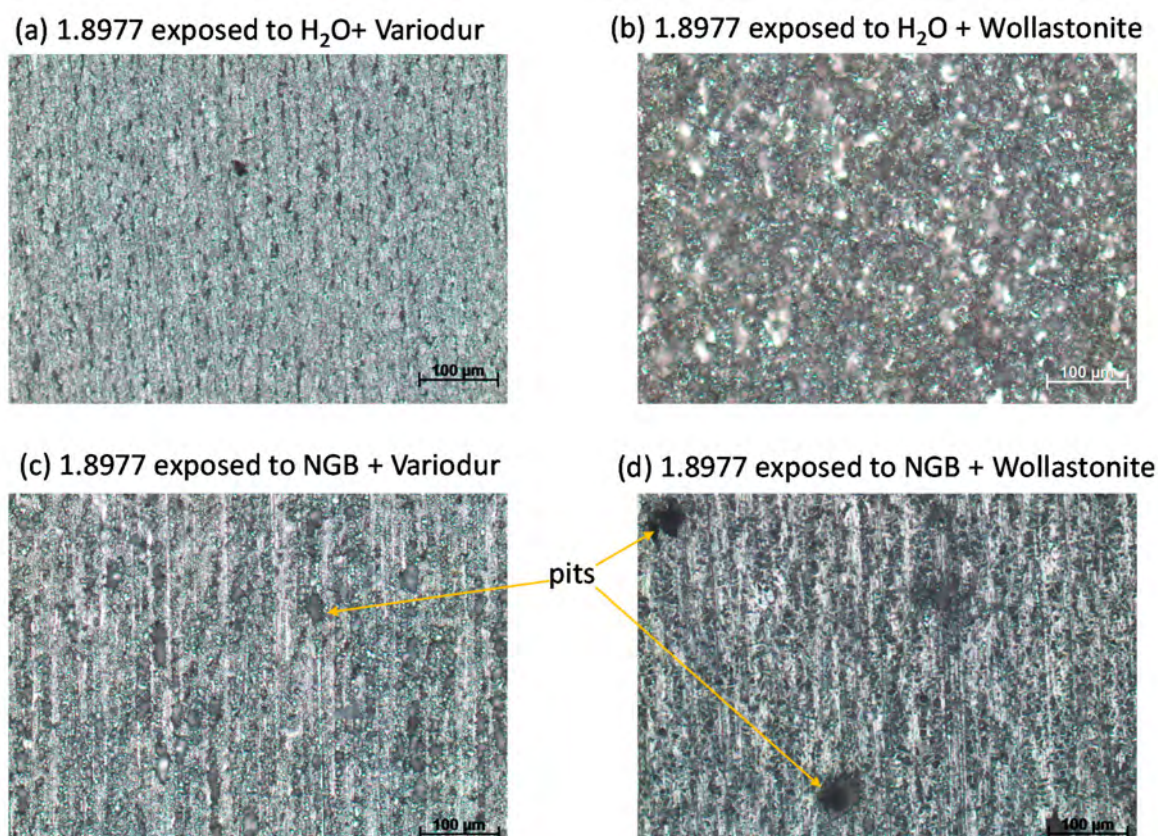
Figure 15. Stereomicroscope images showing the effect of cement on the pitting behavior of 1.8977 in simulated pore water mixed with (c,d) and without (a,b) aquifer fluid NGB.
