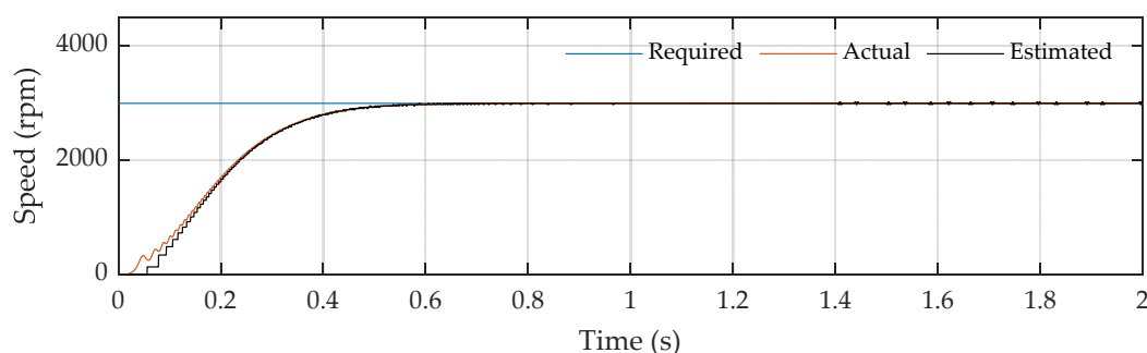
Figure 21. Comparison between the speeds obtained from the simulation model, with a required speed of 3000 rpm.
