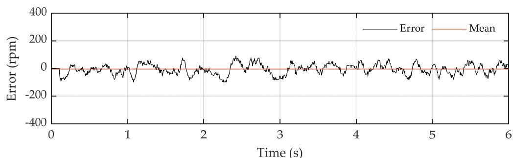
Figure 25. The error between the actual and estimated speeds obtained from the measurement, with a required speed of 3000 rpm.
