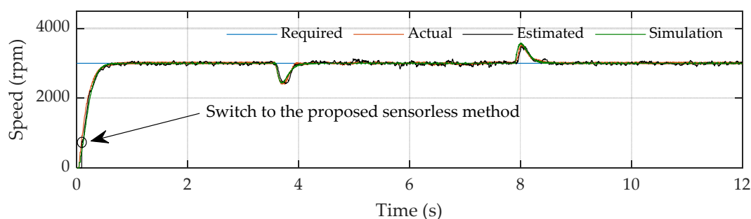
Figure 28. Comparison between the speeds obtained from the measurement and simulation, with a required speed of 3000 rpm and applied load of 0.002 Nm during motor operation.
