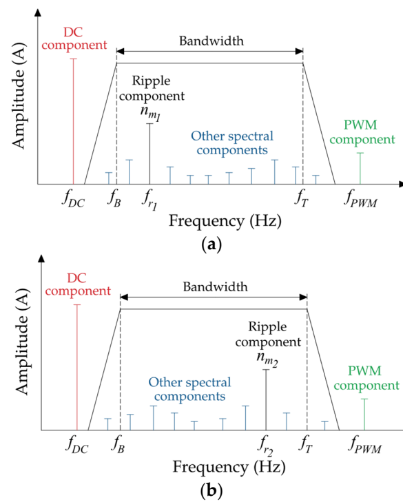
Figure 8. Discrete bandpass filter with fixed bandwidth: (a) the lower rotational speed; (b) the higher rotational speed.
