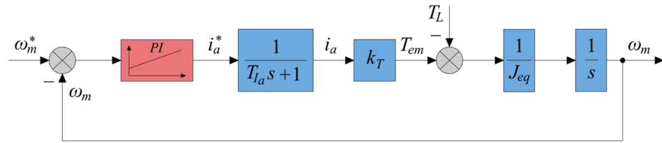
Figure 16. Block diagram of the speed loop.
