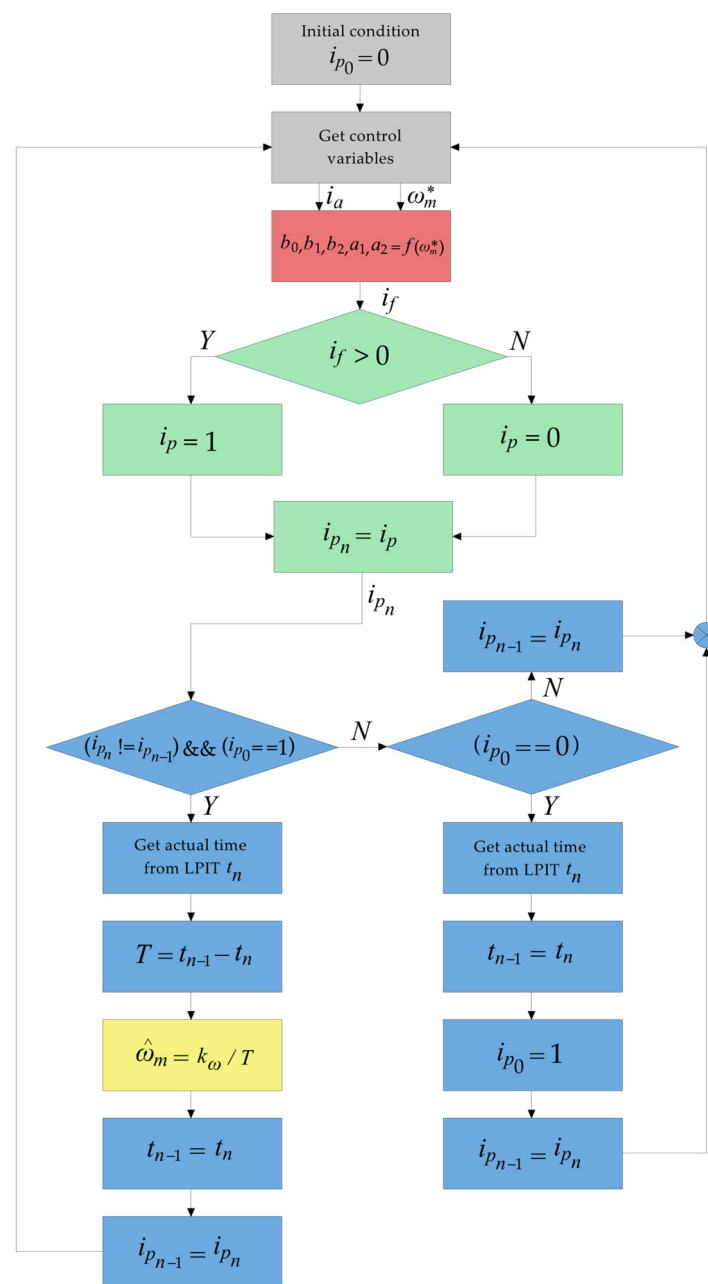
Figure 12. Flowchart of the current signal processing.
