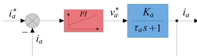
Figure 13. Block diagram of the current loop.
