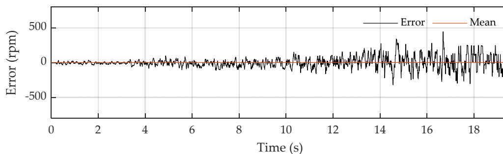
Figure 27. The error between the actual and estimated speeds obtained from the measurement, with stepped changes of required speed from 0 rpm to 6000 rpm.
