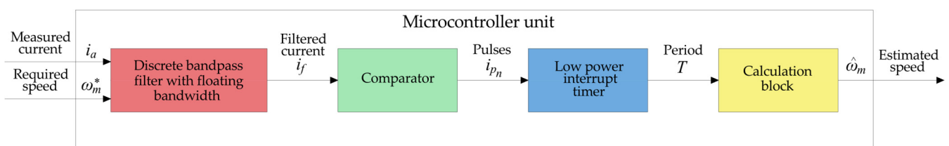
Figure 11. Block diagram of the current signal processing.
