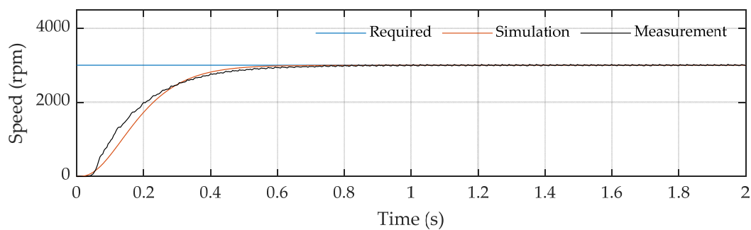
Figure 18. Comparison between the measured and simulated speed, with a required speed of 3000 rpm.
