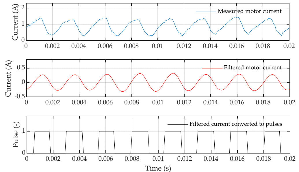
Figure 10. Signal processing of the measured motor current with a rotational speed of 3000 rpm.
