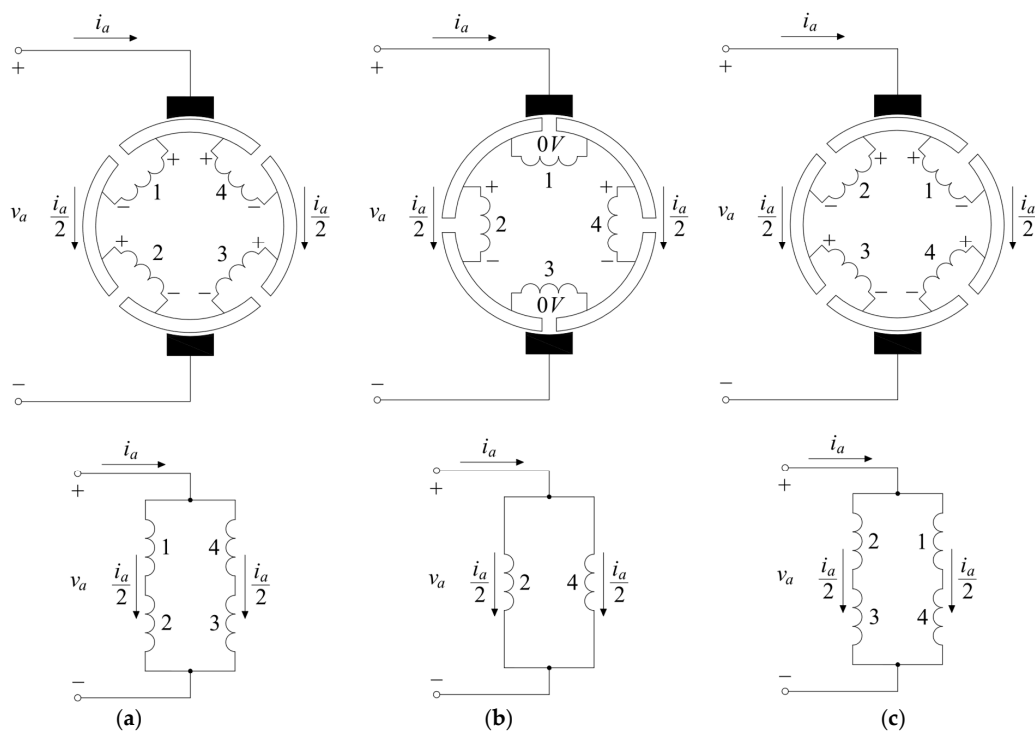
Figure 3. Commutation process of a DC machine with four commutator segments and one pole pair at: (a) \theta_m = 0^\circ ; (b) \theta_m = 45^\circ ; (c) \theta_m = 90^\circ .
