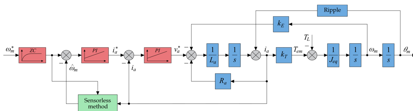
Figure 20. Block diagram of the proposed sensorless control.
