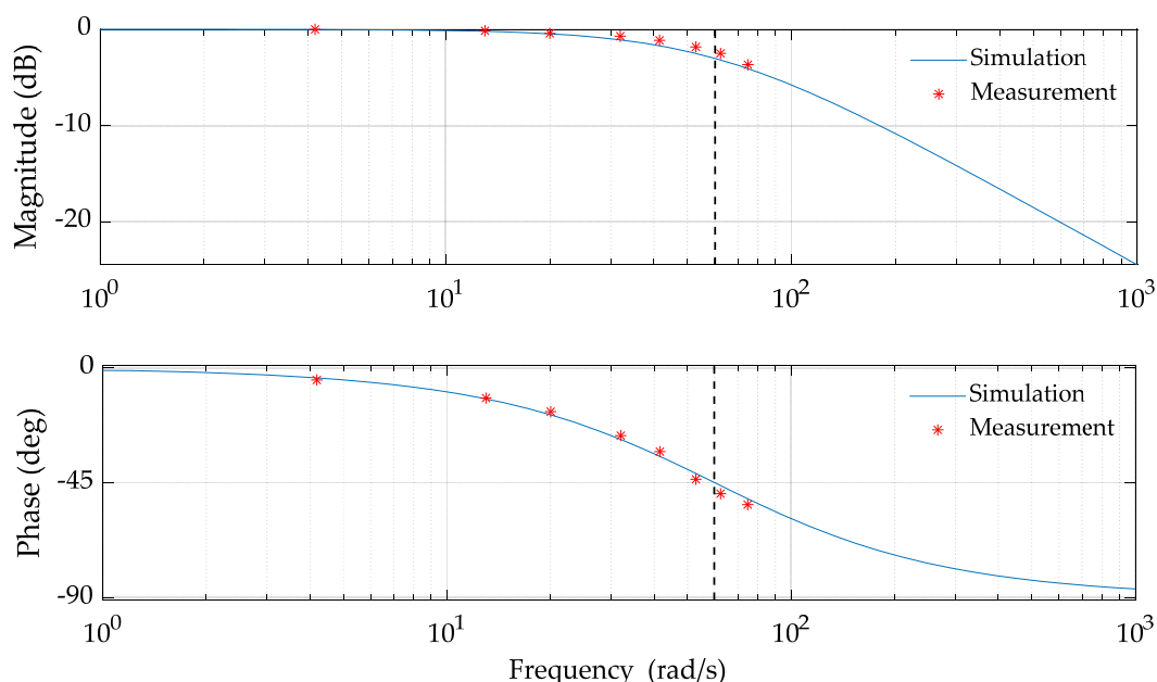
Figure 15. Bode plot of the current loop frequency response.
