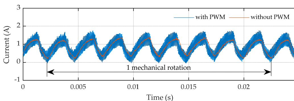
Figure 5. Brushed DC motor current—comparison.
