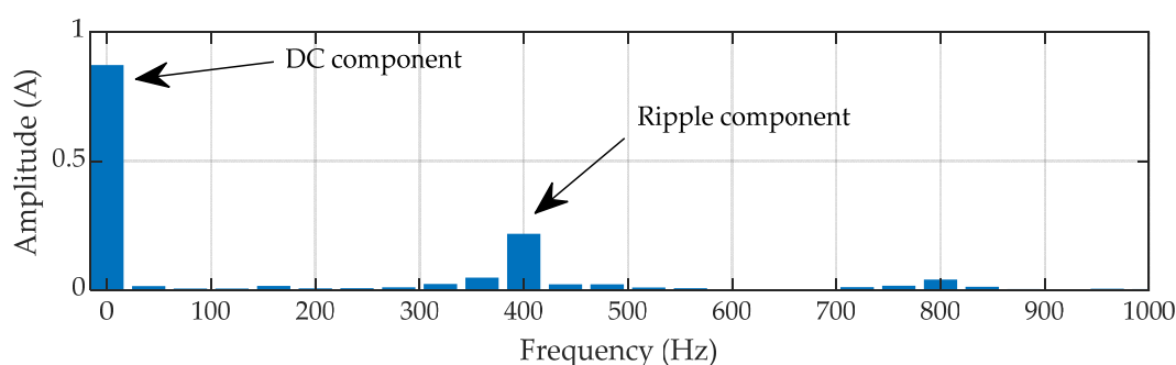
Figure 6. Brushed DC motor current in the frequency domain—DC component and ripple component.
