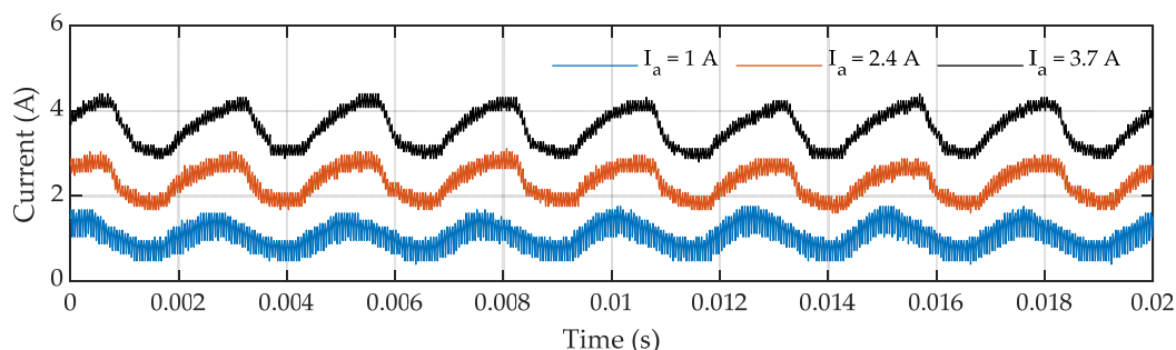
Figure 30. The brushed DC motor current at three different load conditions with a rotational speed of 3000 rpm.
