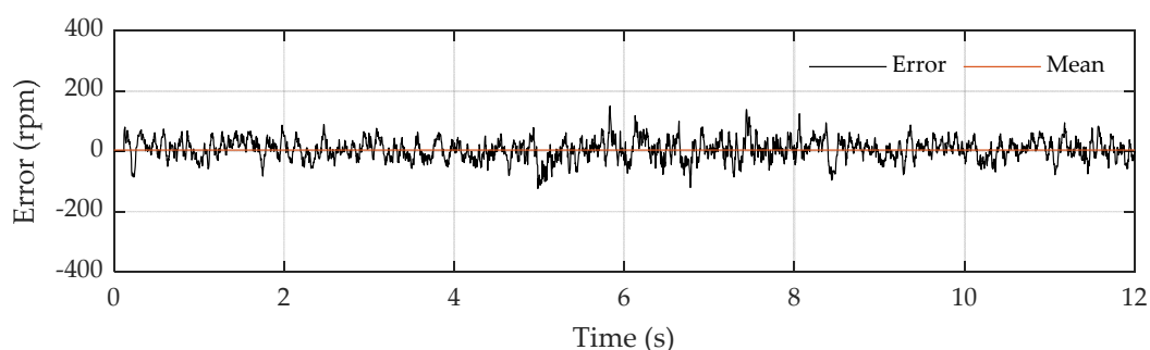
Figure 29. The error between the actual and estimated speeds obtained from the measurement, with a required speed of 3000 rpm and applied load of 0.002 Nm during motor operation.
