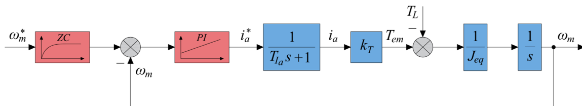
Figure 17. Block diagram of the speed loop with the zero cancellation.
