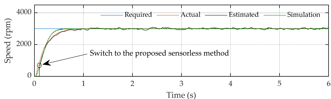
Figure 24. Comparison between the speeds obtained from the measurement and simulation, with a required speed of 3000 rpm.
