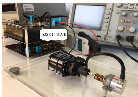
Figure 23. Photo of the experimental setup.
