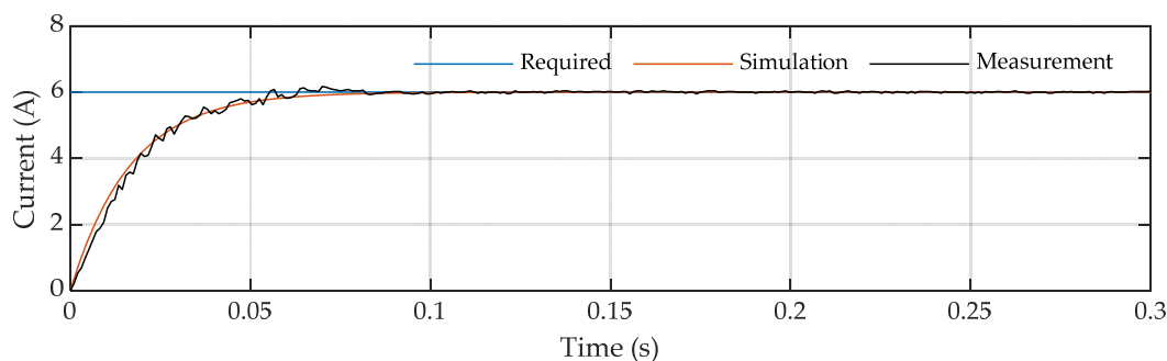
Figure 14. Comparison between the measured and simulated current, with a required current of 6 A.
