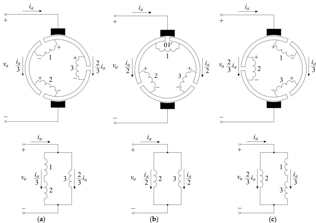
Figure 4. Commutation process of a DC machine with three commutator segments and one pole pair at: (a) \theta_m = 0^\circ ; (b) \theta_m = 30^\circ ; (c) \theta_m = 60^\circ .
