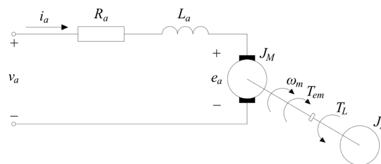
Figure 1. Equivalent circuit of DC motor.
