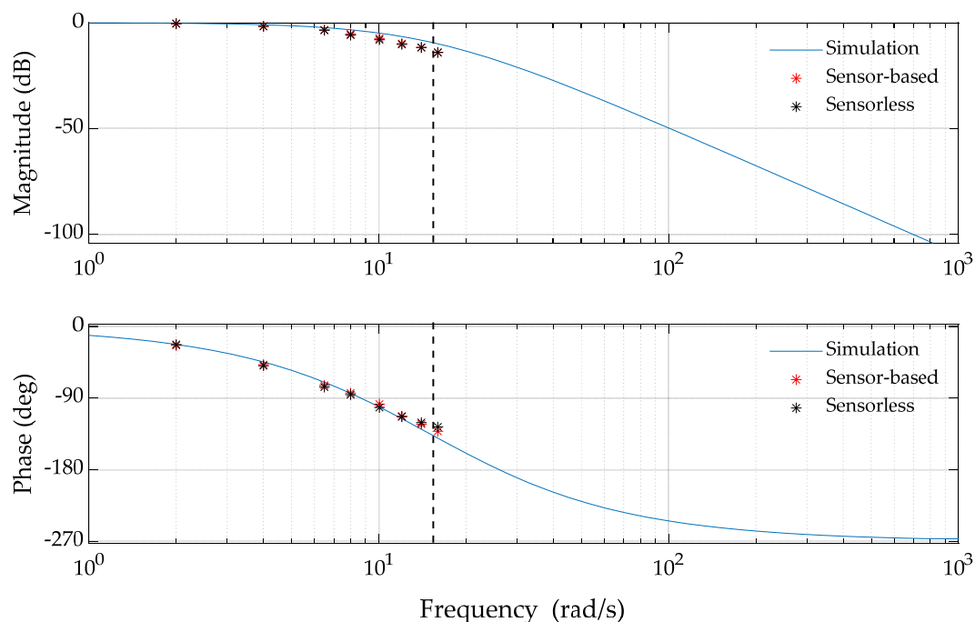
Figure 31. Bode plot of the speed loop frequency response for sensor-based and sensorless.
