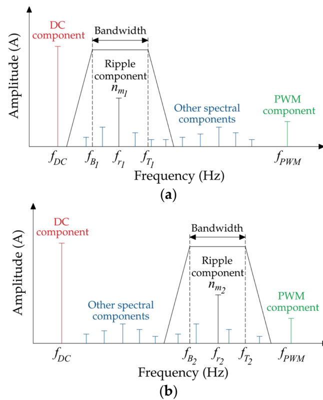
Figure 9. Discrete bandpass filter with the floating bandwidth: (a) the lower rotational speed; (b) the higher rotational speed.
