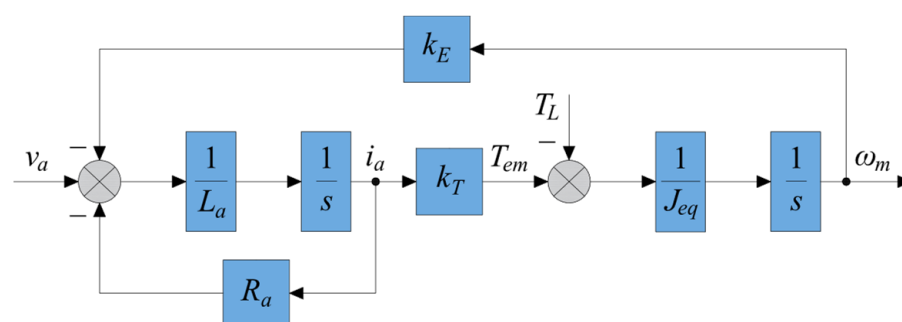
Figure 2. Block diagram of DC motor.
