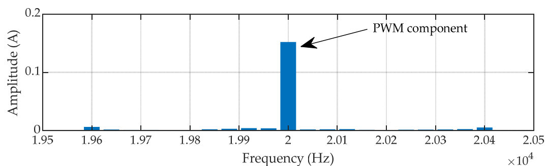
Figure 7. Brushed DC motor current in the frequency domain—PWM component.
