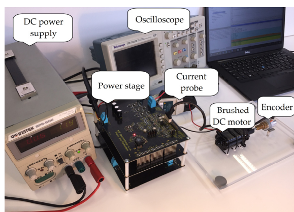
Figure 22. Photo of the experimental setup.
