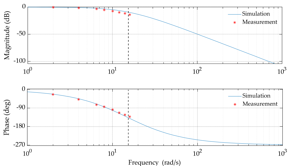
Figure 19. Bode plot of the speed loop frequency response.
