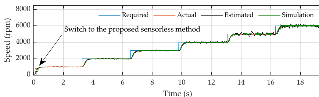
Figure 26. Comparison between the speeds obtained from the measurement and simulation, with stepped changes of required speed from 0 rpm to 6000 rpm.
