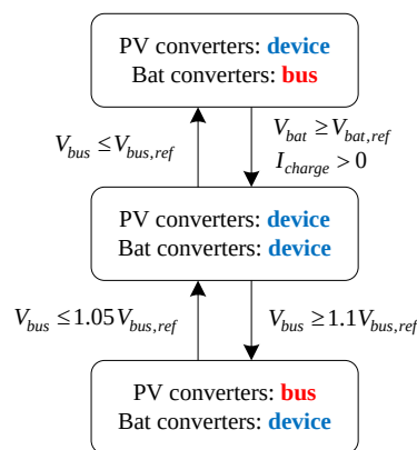
Figure 2. Diagram of the transitions between bus-regulating mode and device-regulating mode.
