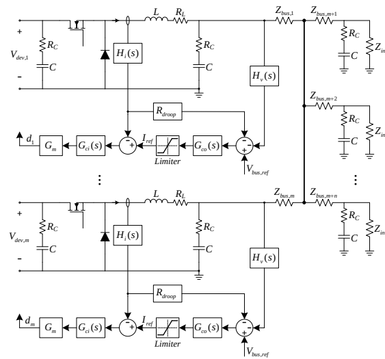
Figure 10. The control block diagram of bus-regulating converters.
