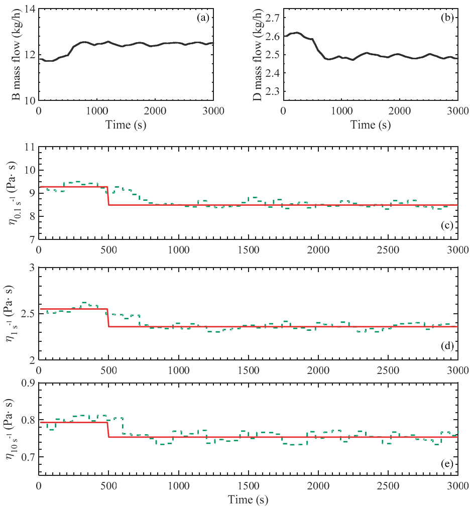
Figure 10. Performance of controller for the case with time sampling equal to 60 s: (a) mass flow of ingredient B; (b) mass flow of ingredient D; (c) response of the viscosity at shear rate equal to 0.1 \text{ s}^{-1} ; (d) response of the viscosity at shear rate equal to 1 \text{ s}^{-1} ; (e) response of the viscosity at shear rate equal to 10 \text{ s}^{-1} . For (c–e) the following data are reported: target curve (red solid line), measured value (green dashed line).
